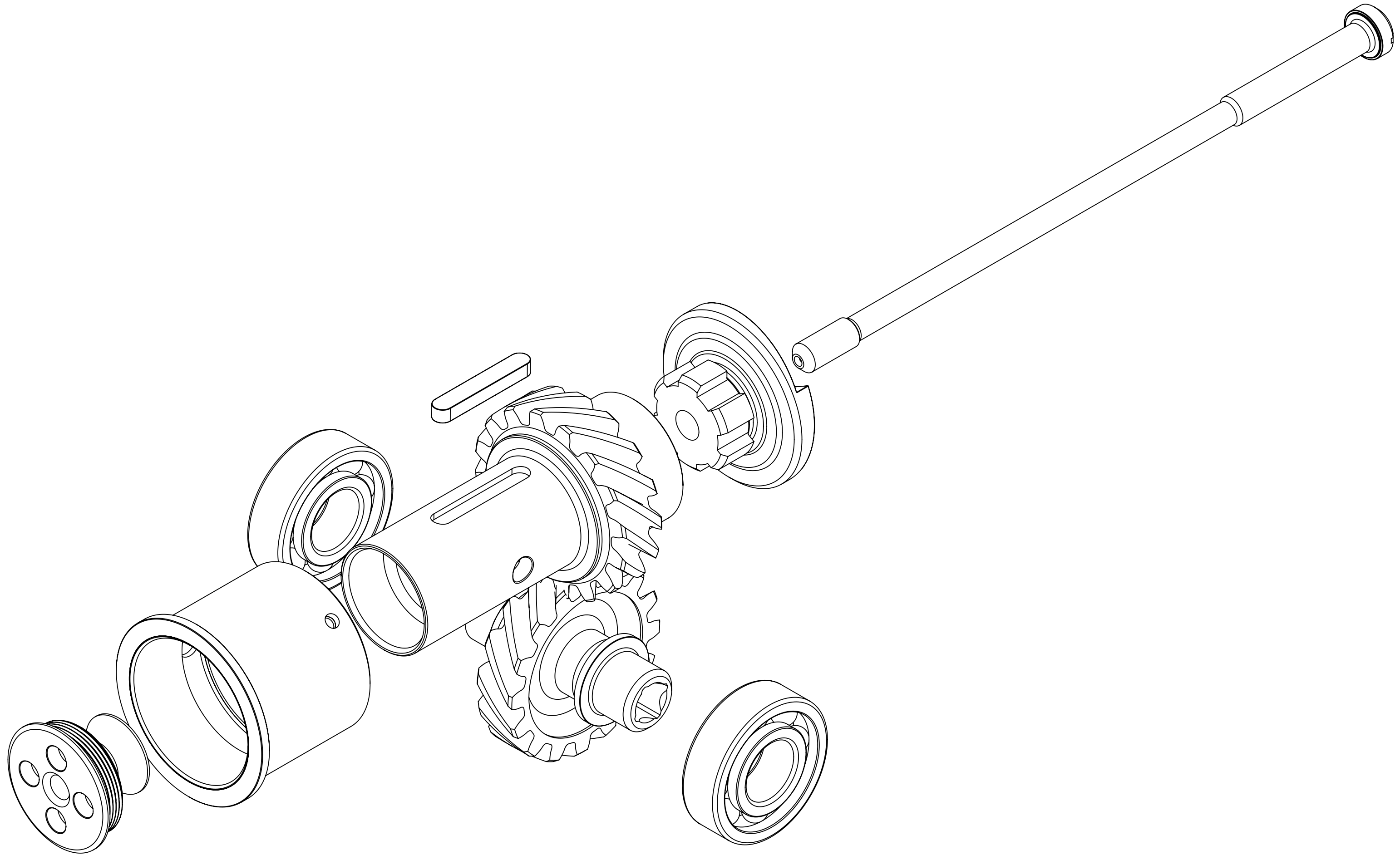
Wright J-5 Auxiliary Drive Gears. J Riend 30nov23
